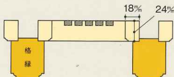
KM-5 [二重格縁付吹寄せ小組格天組立品]
