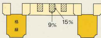
KM-2 [二重格縁付小組天井組立品]
